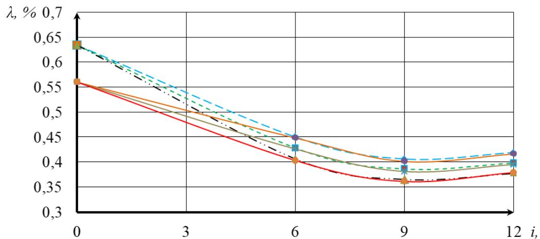
Figure 2. The graph of dependence of the wear level of the outer cylinder of the sliding bearing on the longitudinal and oblique longitudinal grooves opened to the inner cylinder.
