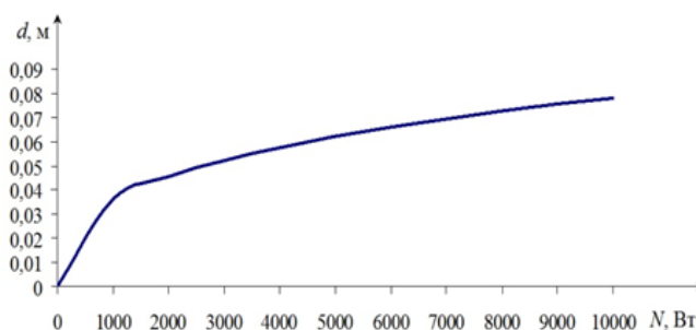
Figure 1. The graph of the transmitted power as a function of the diameter of the wheel shaft
