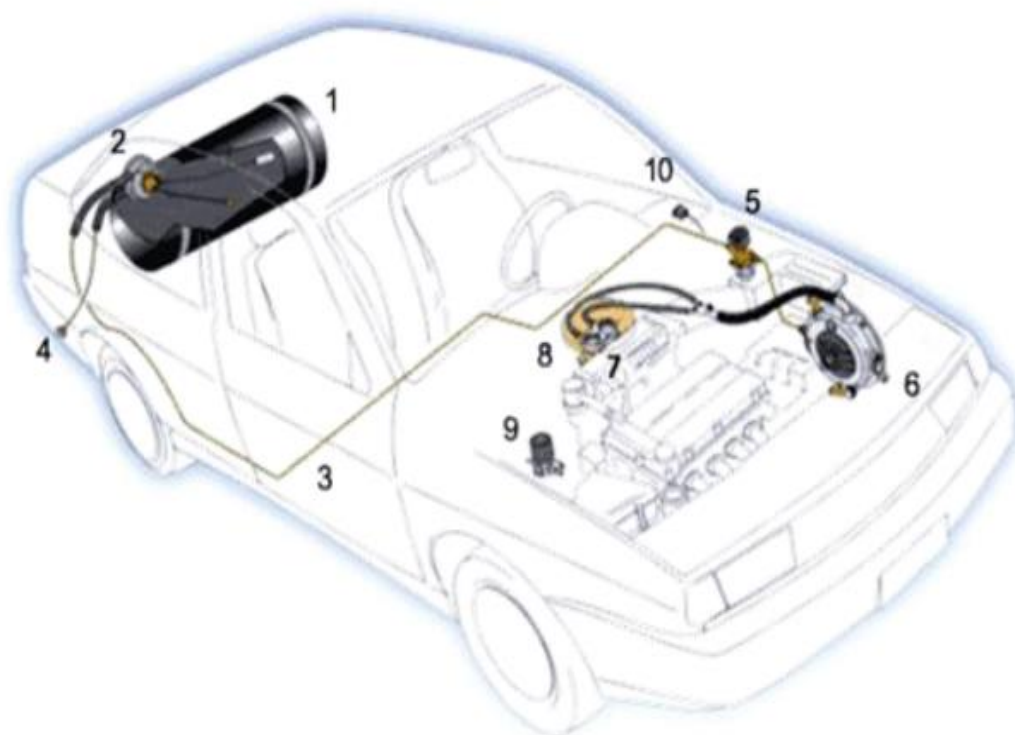
Figure 1. Cars with liquefied gas supply system
