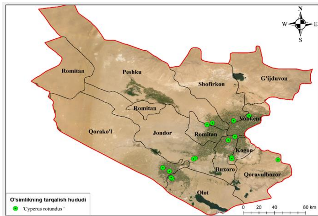
Figure 1. The distribution of Cyperus rotundus in Bukhara region.
